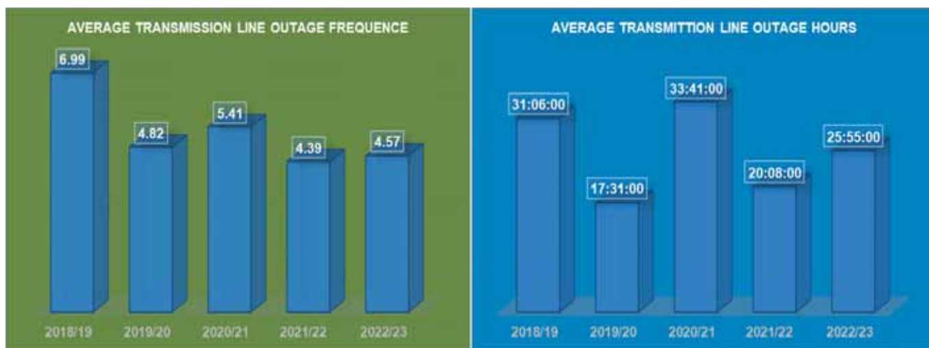
Figure 52: Average Transmission Line Outage Hours and Frequency
